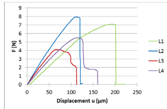
FIGURE 6. Tensile force versus displacement ( \mu\text{m} ). There are two types of behavior: the fragile behavior with sudden rupture (the blue and the green curve) and the behavior with partial resistance of the wood filament after the initial yield (the red curve and the violet curve).
